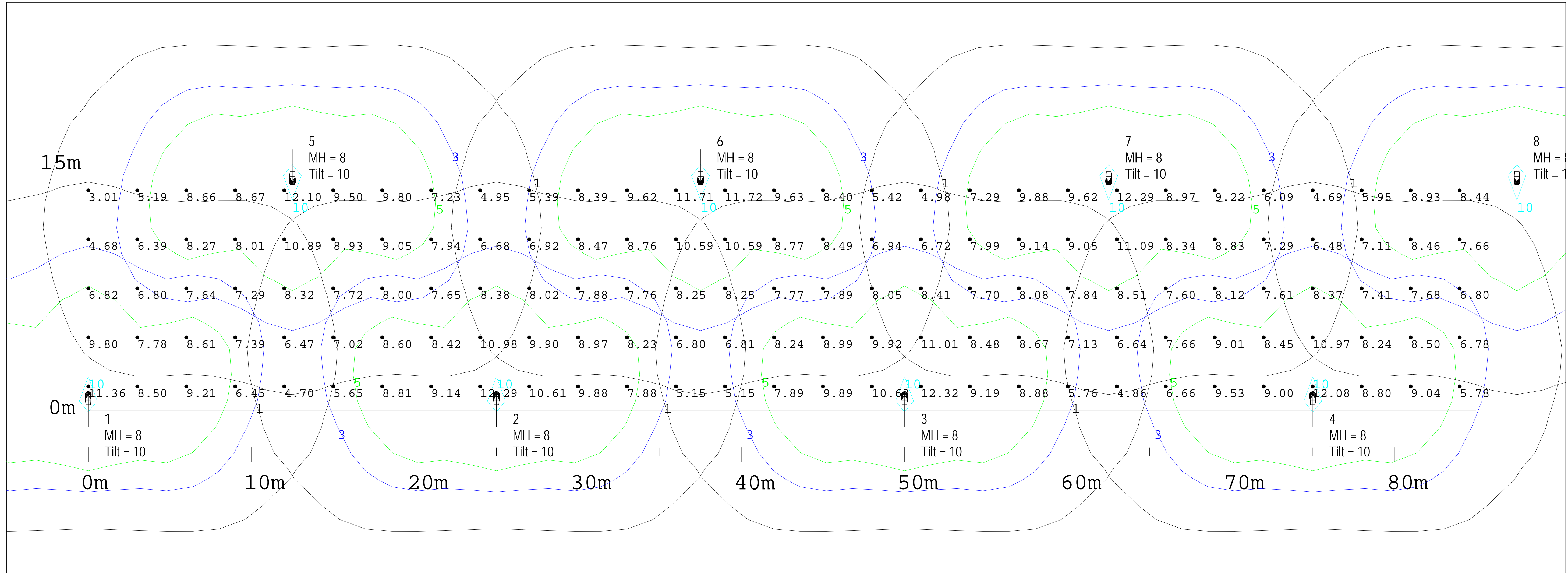
15m Wide Sample Roadway (1m Setback) 8m Mounting Height and 25m Staggered Spacing Scale: None
